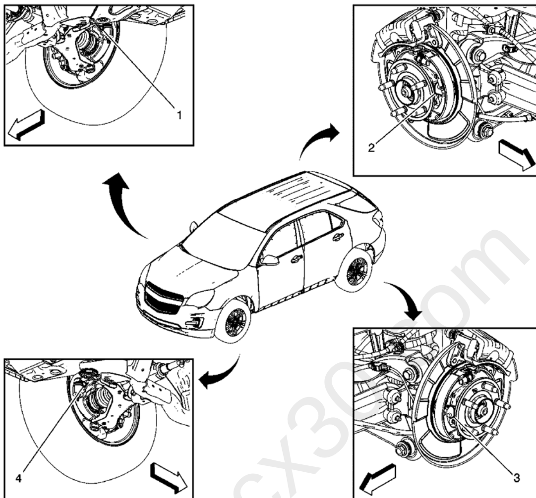
Fig. 2: Locating Wheel Components Courtesy of GENERAL MOTORS CORP.
